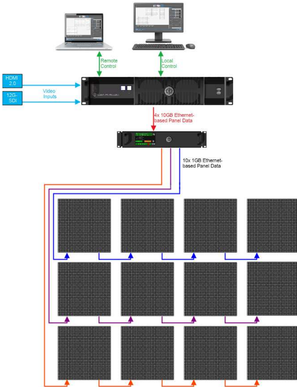
Figure 2-2. Typical system set-up for SX40 processor
