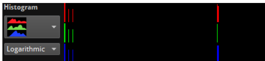
Figure 9-4. Test pattern showing colour bars at 75% and the corresponding Logarithmic RGB histogram
