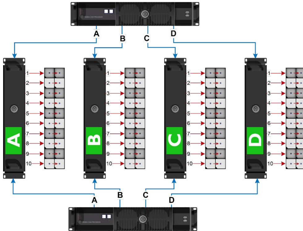
Figure 4-5. Processor redundancy
