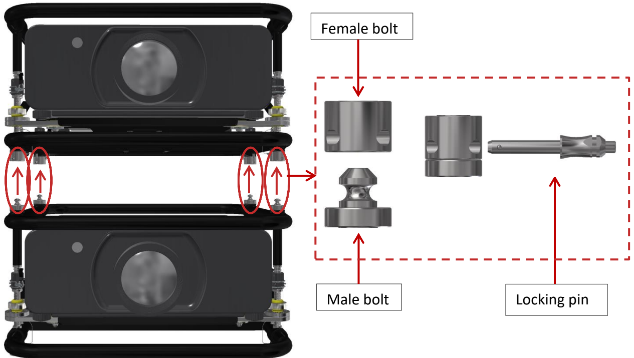
Figure 20 Stacking frames
