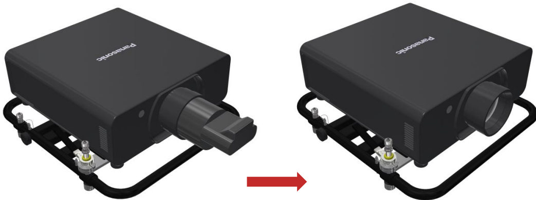
Figure 12 Remove the ultra-short throw lens
