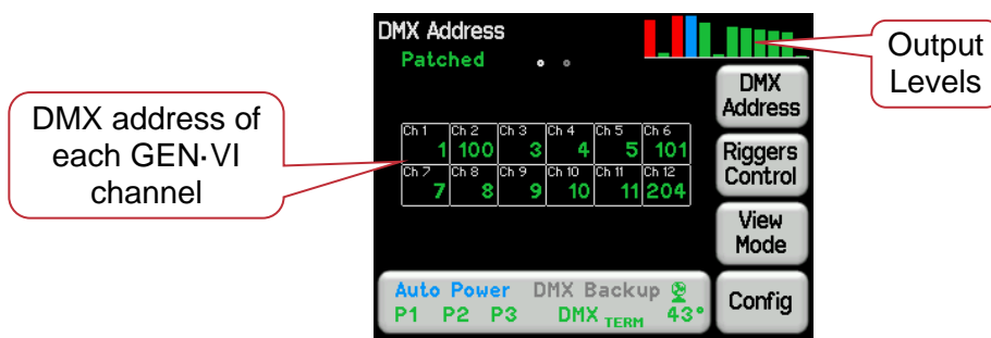
“DMX Address” Home Page with channels individually patched
