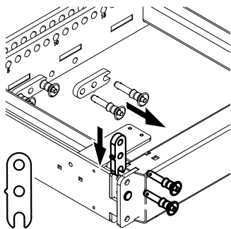
Splay link of the frame – «POSITION Y8/Y12»
