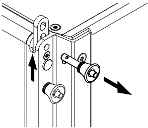
Y-SUB Front link mechanism
