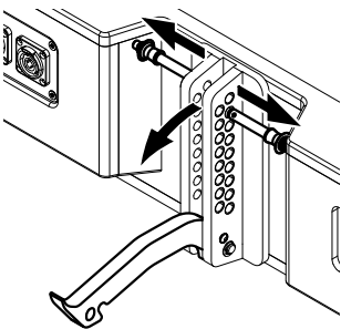
Splay/Rear link mechanism
