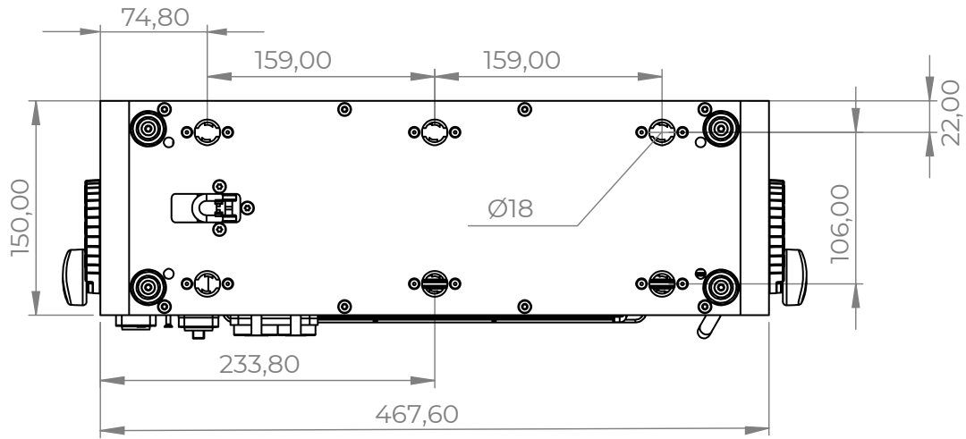
Figure 2: Dimensions for base locking points
